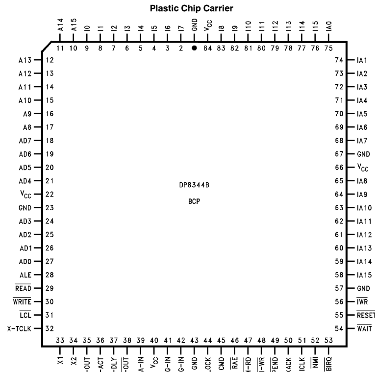
FIGURE 5-1. Top View
