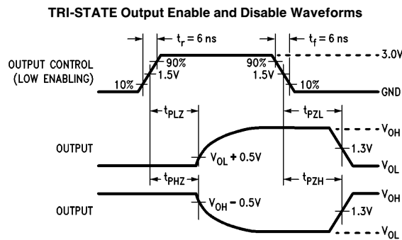
FIGURE 5-2. Switching Characteristic Measurement Waveforms
