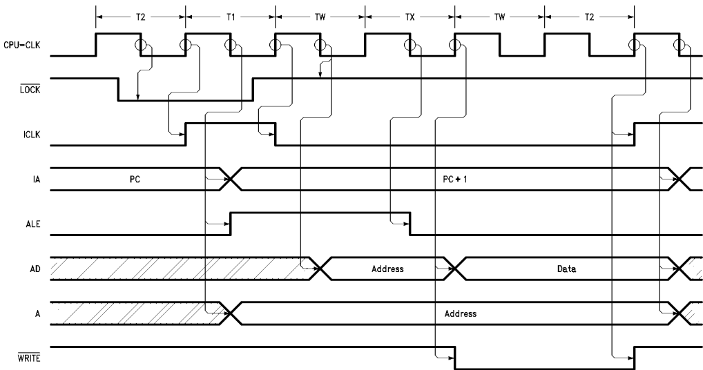
FIGURE 2-31. LOCK Timing with One Wait State
