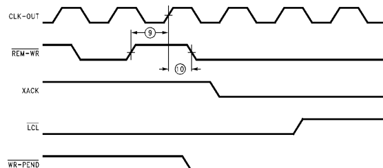
(e) REM-WR Rest Time (Latched Write Mode)
