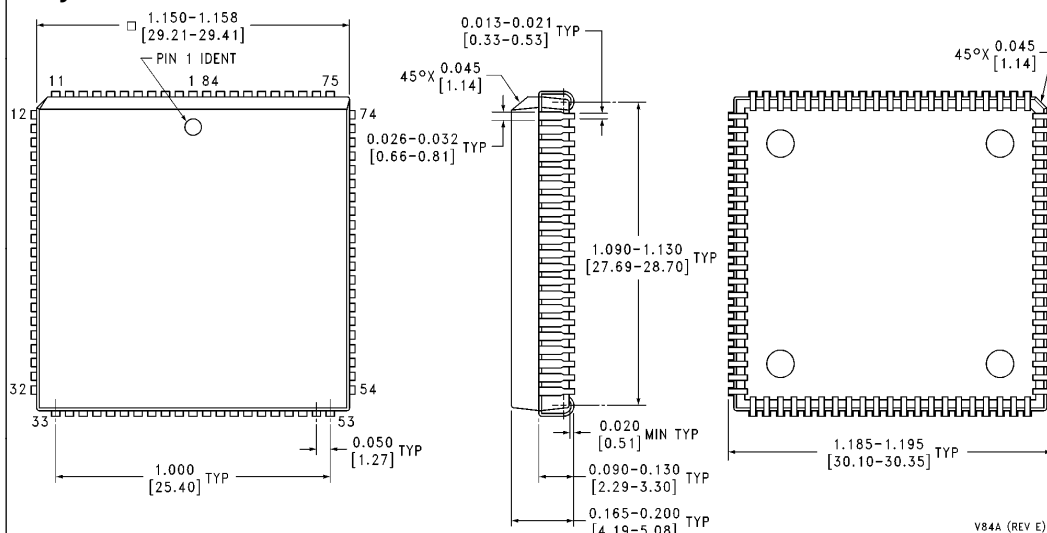
Plastic Chip Carrier (V) Order Number DP8344B NS Package Number V84A
