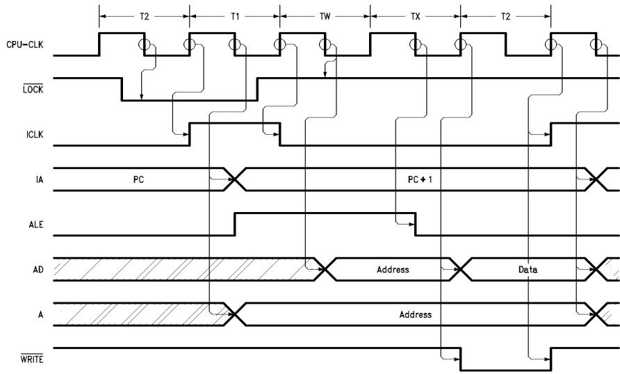
FIGURE 2-30. LOCK Timing
