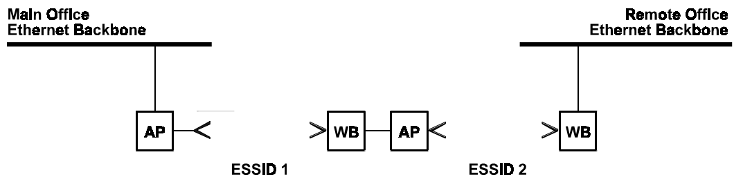
Figure 5-6. Multi-Hop Configuration
