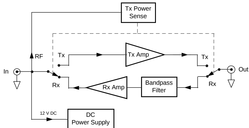
Figure 6-5. AMP 2440 Functional Block Diagram
