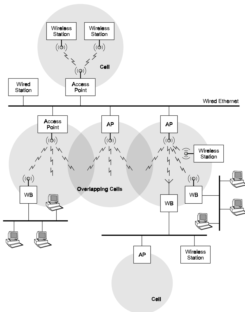
Figure 9-3. Wireless LAN Connectivity
