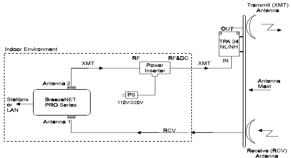
Figure 6-1. TPA 24 Installation
