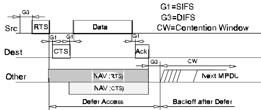
Figure 9-15. Transaction Between Stations A and B
