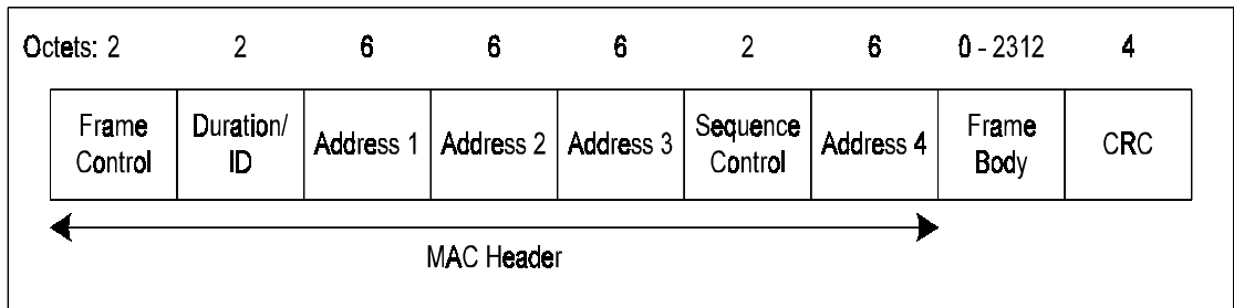
Figure 9-18. MAC Frame Format
