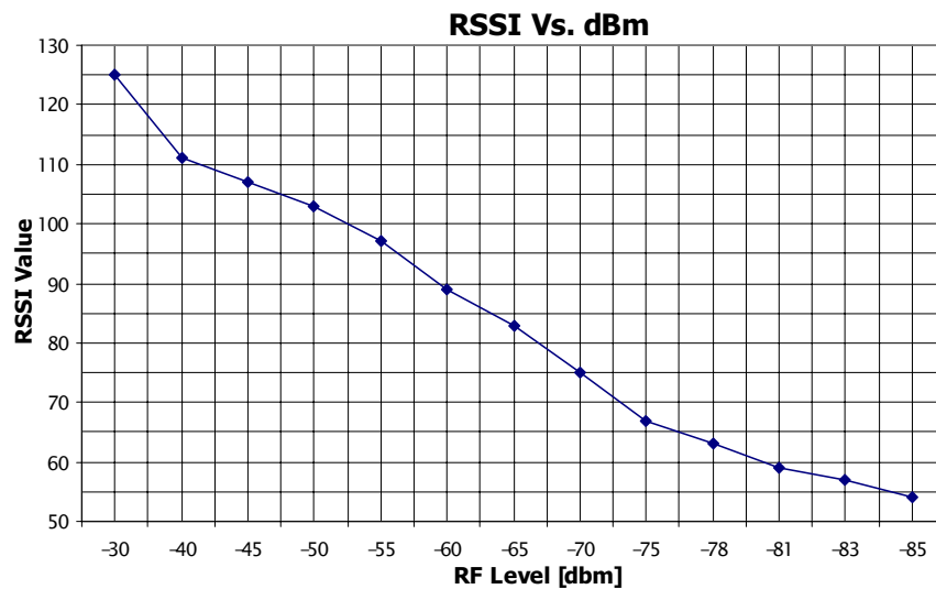
Figure 3-8. RSSI to dBm Graph
