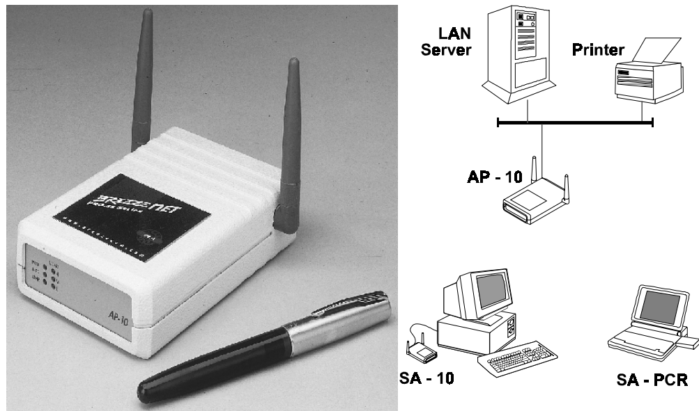
Figure 1-1. AP-10 PRO.11 with Two Built-in Omni-Directional Antennas
