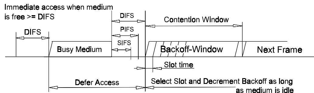
Figure 9-17. Access Mechanism
