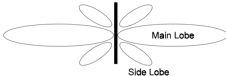
Figure 9-8. Side View
