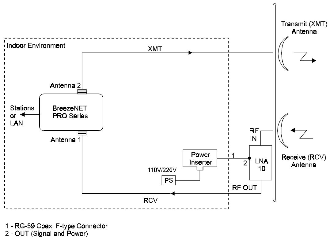
Figure 6-2. LNA 10 Connections Diagram
