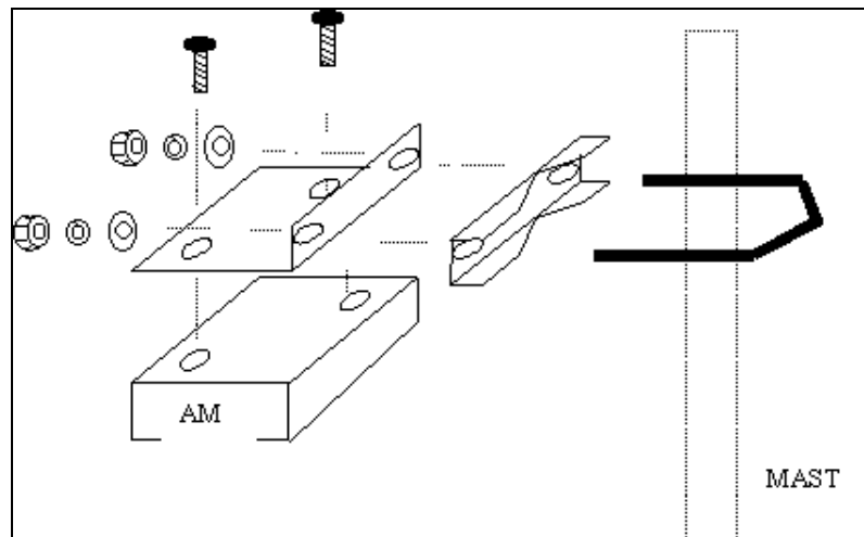
Figure 6-6. AMP 2440 Installation and Mounting
