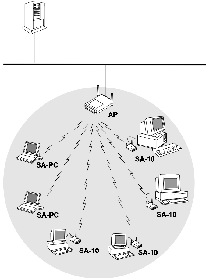
Figure 5-3. Single Cell Configuration
