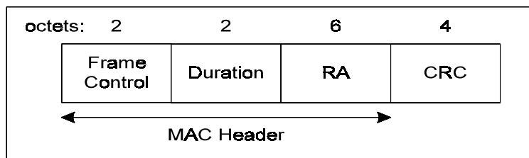
Figure 9-22. ACK Frame Format
