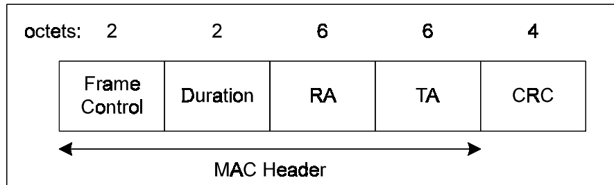
Figure 9-21. CTS Frame
