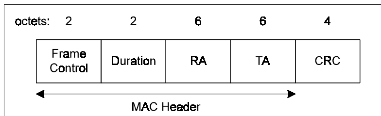
Figure 9-20. RTS Frame Format
