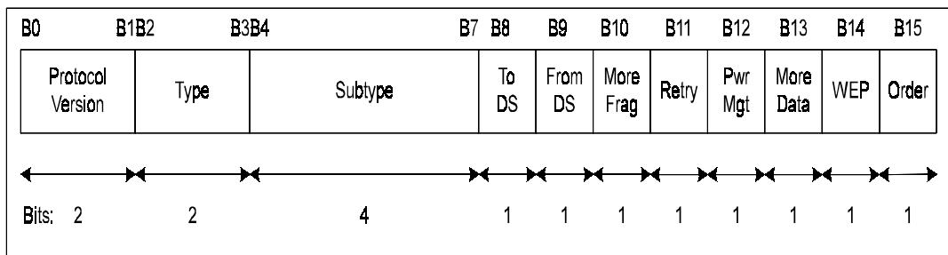
Figure 9-19. Frame Control Field
