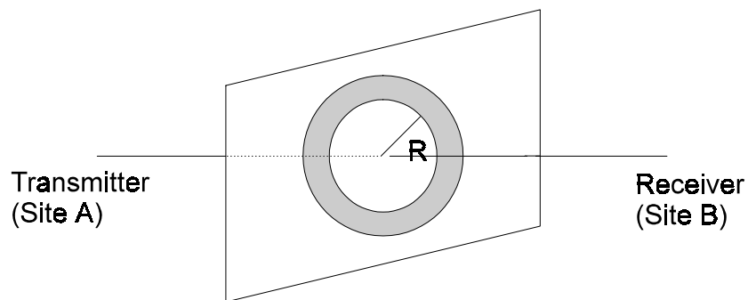
Figure 9-12. Fresnel Zone
