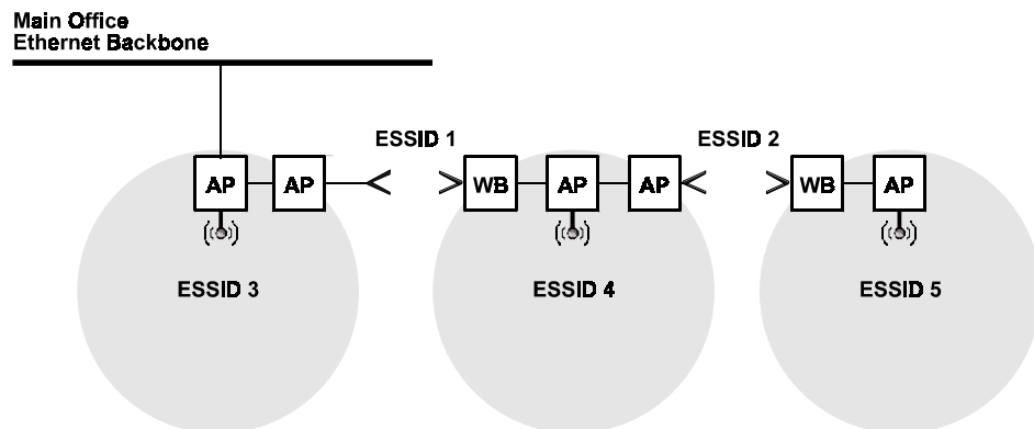
Figure 5-7. Advanced Multihop Configuration
